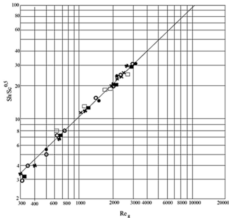
Fig. 1: Comparison of calculated and experimental mass transfer data in the gaseous phase Experimental data : □, ○, × - tube with an extended neck; ■, ●, * - Venturi tube; ×, * - type 1; ○, ● - type 2; □, ■ - type 3; Line – calculations from formula (5)
