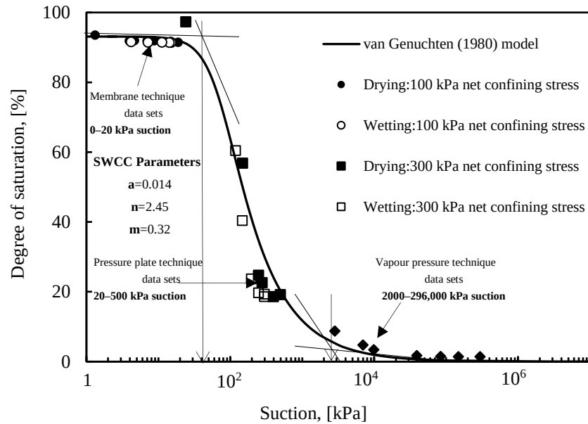
Figure 5. Curve fitting of soil-water characteristic curve data sets with different stress conditions.
