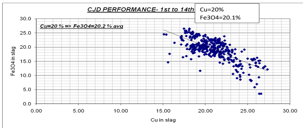
Figure 7: Performance of the Angular distributor Ring for the period 1 st to 14 th May
