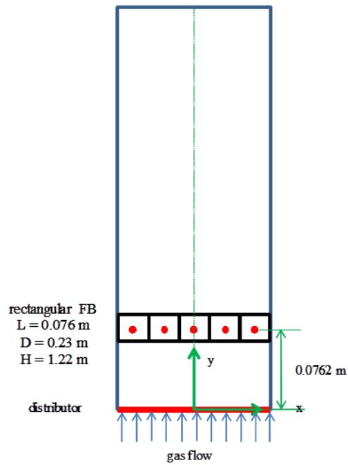
Fig 1: NETL SSCP1 experimental test rig
