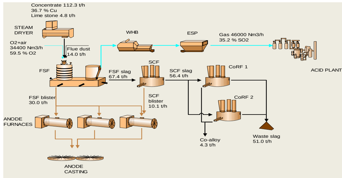
Figure 1: Flowsheet of the Direct-to-Blister Process at Nchanga Smelter (Outotec 2010)
