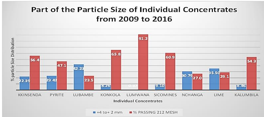
Figure 3: Individual concentrates particle size distribution for the period 2009 to 2016
