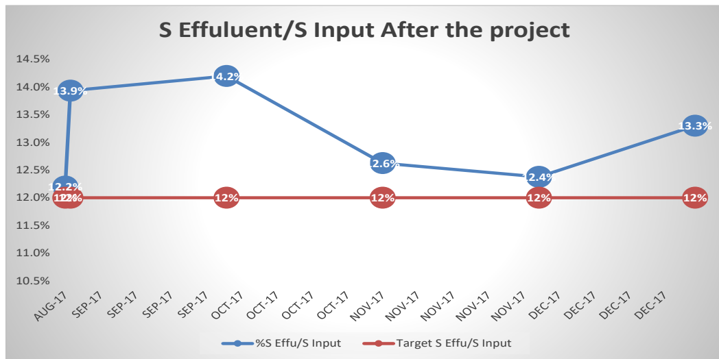
Figure 13: Comparison of sulphur in feed and effluent after the project
