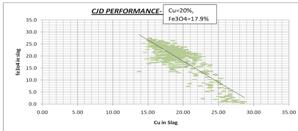
Figure 8: Performance of the Tangential distributor Ring for the period 14 th to 31 st May
