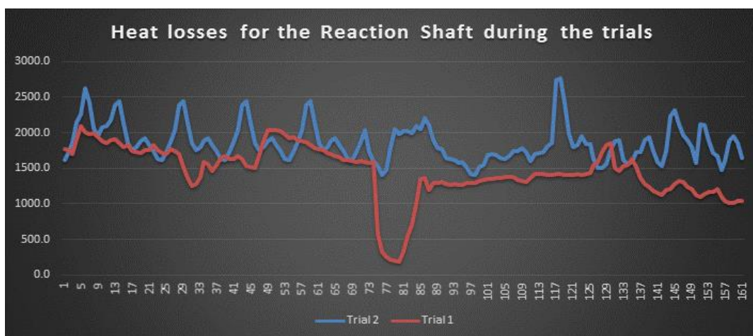
Figure 11: Heat Losses (KW) in the reaction shaft during the trial period
