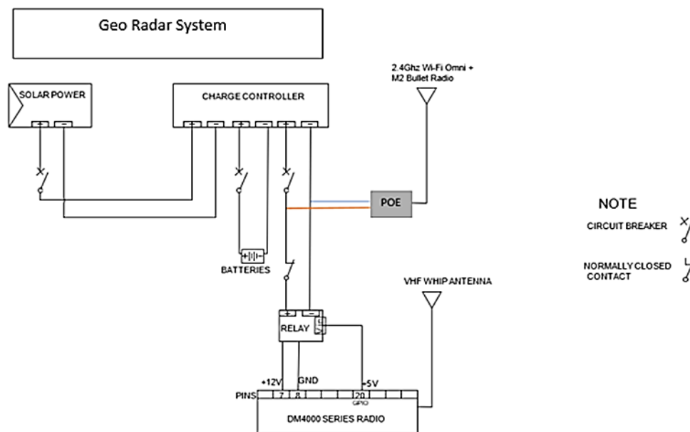
Fig. 3: Connection layout
