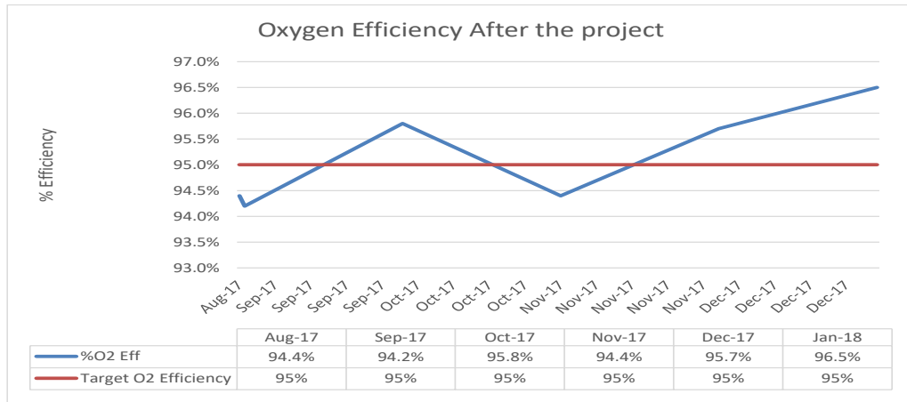
Figure 12: Oxygen efficiency after the project
