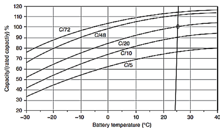
Figure 2. Lead-acid battery capacity depends on discharge rate and temperature. The capacity at C/20 and 25°C.( Masters, 2013)
