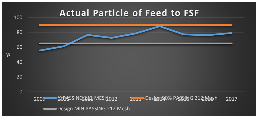
Figure 4: Particle size distribution for FSF feed
