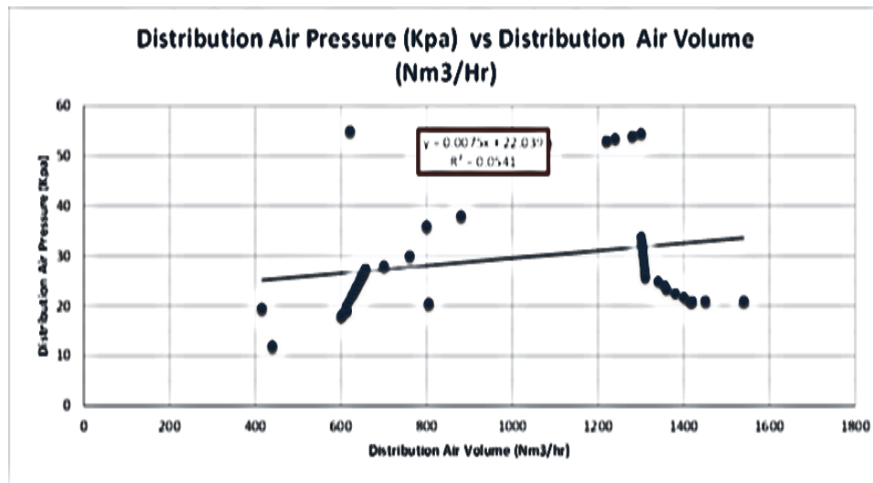
Figure 9: Comparison of distribution air pressure and Volume
