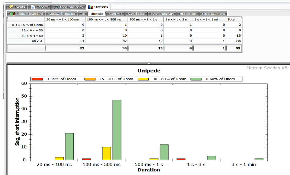
Figure 9: UNIPEDE graph showing dips with durations and depths. (Source: Metrum AB, 2021)
