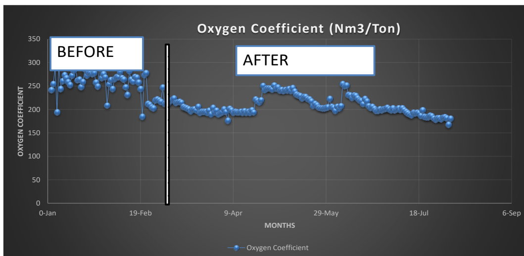
Figure 14: Comparison of oxygen efficiency before and after the project
