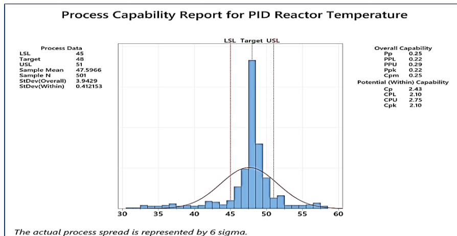
Figure 5b: Process capability report for PID controller
