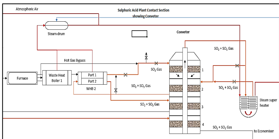
Figure 1: SAP Contact Section showing Catalytic Converter Beds 1-4
