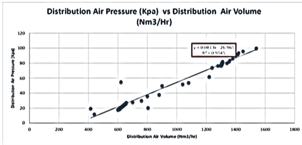
Figure 10: Comparison of distribution air pressure and Volume
