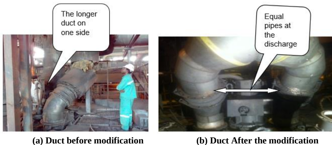
Figure 5: Oxygen duct design before and after modifications
